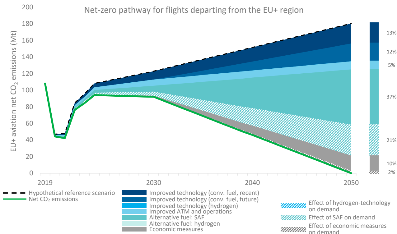
Figure 7: Overall impacts on net CO 2 emissions (TtW) of intercontinental flights departing the EU+ region, for 2030, 2040 and 2050. Sustainability measures are not assessed year by year, as such pathways and contributions of individual measures may differ from the linear interpolation shown in the graph
